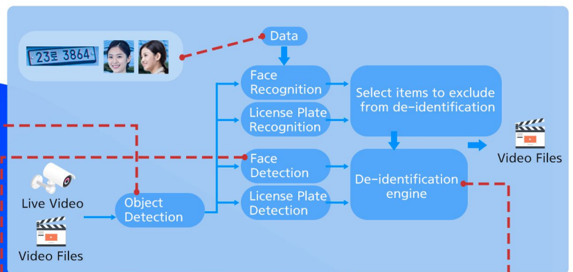
2 Metadata extraction
